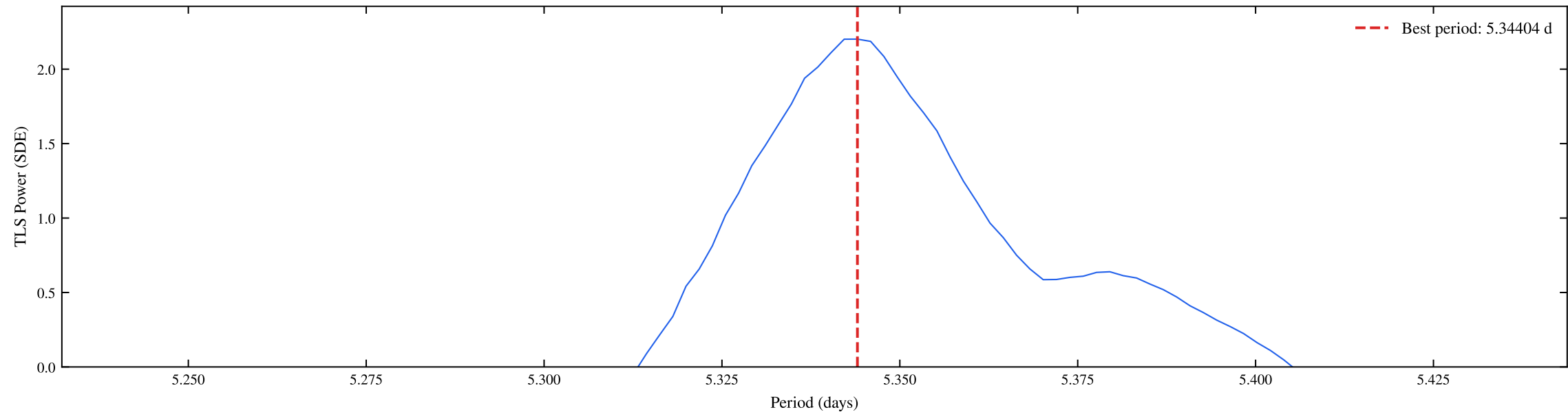
TIC 128790976 | Sectors: 13 | TLS Fine Periodogram (SDE = 2.20)
