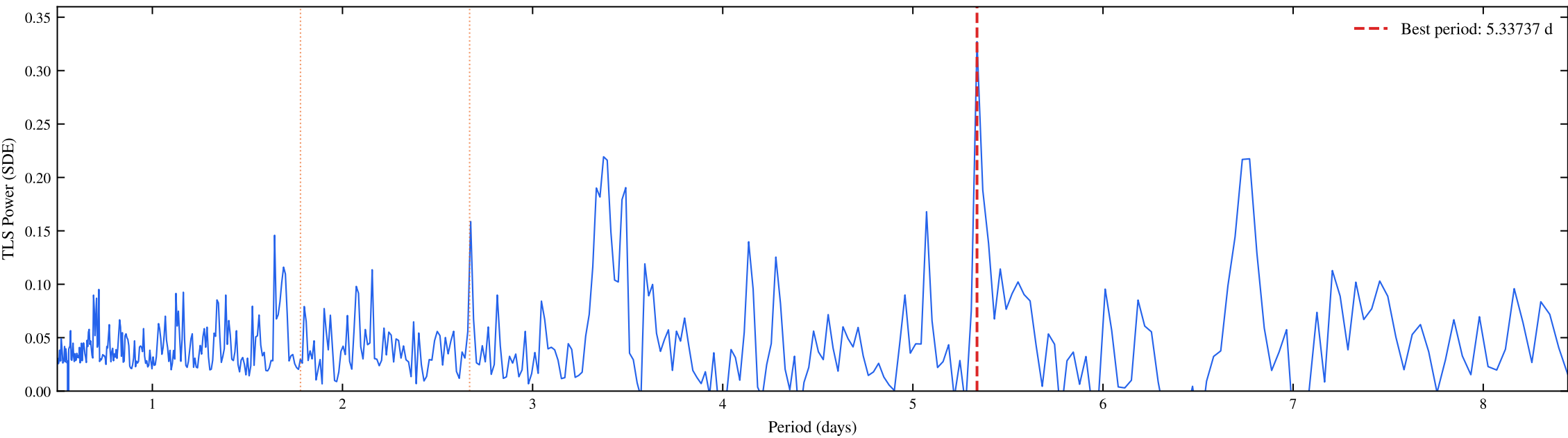
TIC 128790976 | Sectors: 13 | TLS Periodogram (Planet 2 Search) (SDE = 0.33)
