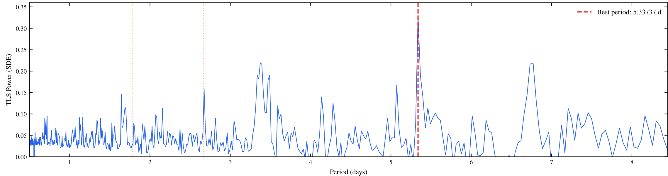
TIC 128790976 | Sectors: 13 | TLS Coarse Periodogram (SDE = 0.33)
