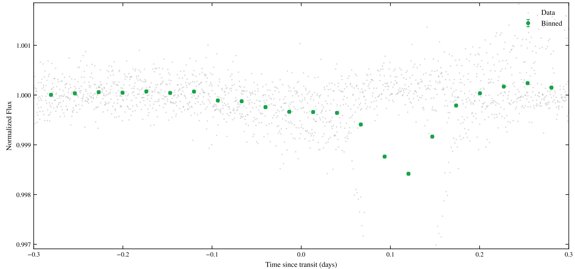
TIC 128790976 | Sectors: 13 | Phase-Folded Transit (P = 5.34404 d)
