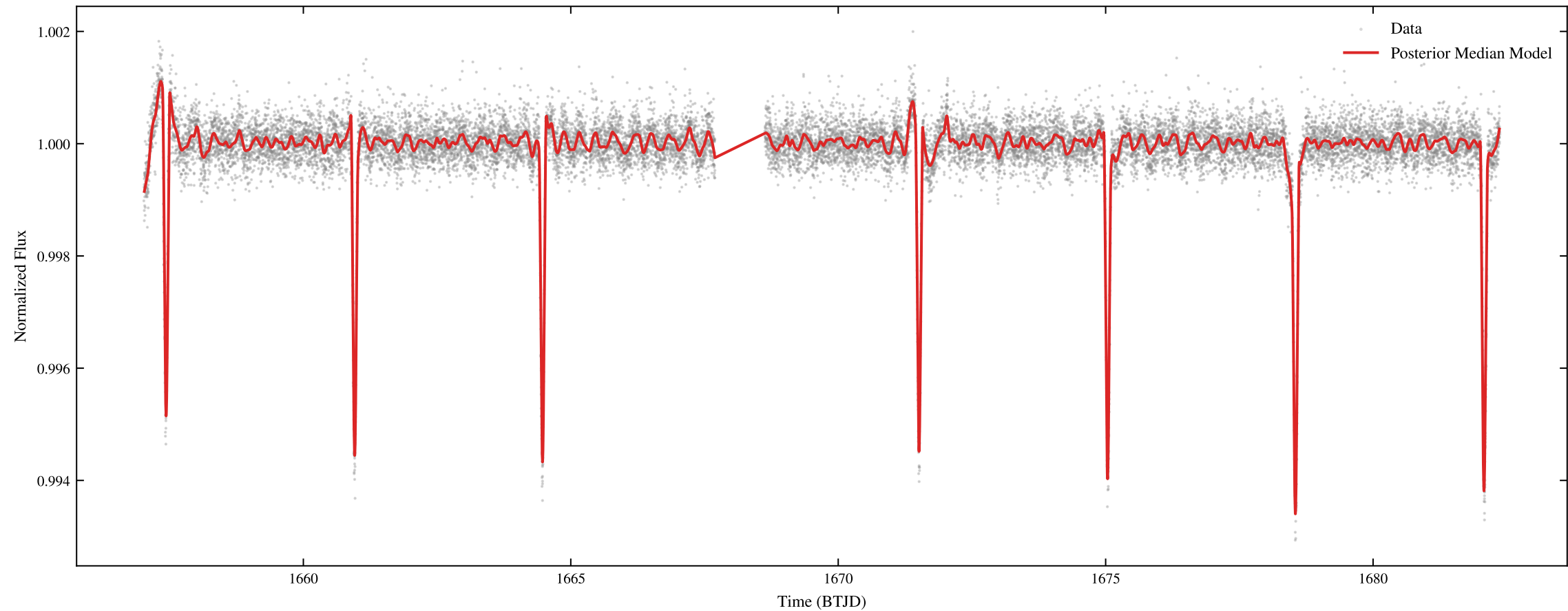
TIC 128790976 | Sectors: 13 | MCMC Posterior Predictive Check
