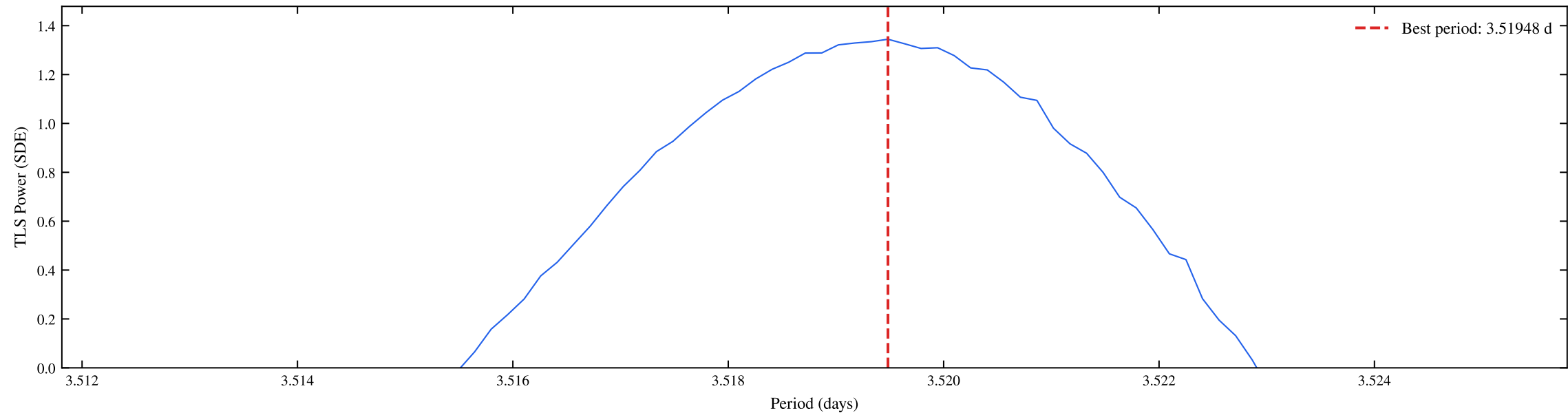
TIC 128790976 | Sectors: 13 | TLS Fine Periodogram (SDE = 1.34)
