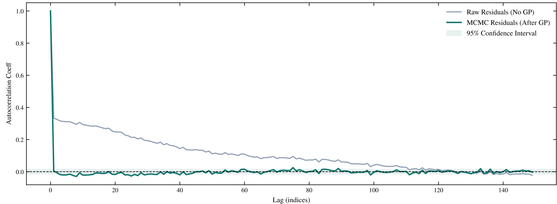
TIC 128790976 | Sectors: 13 | GP Residuals Autocorrelation Function (ACF)
