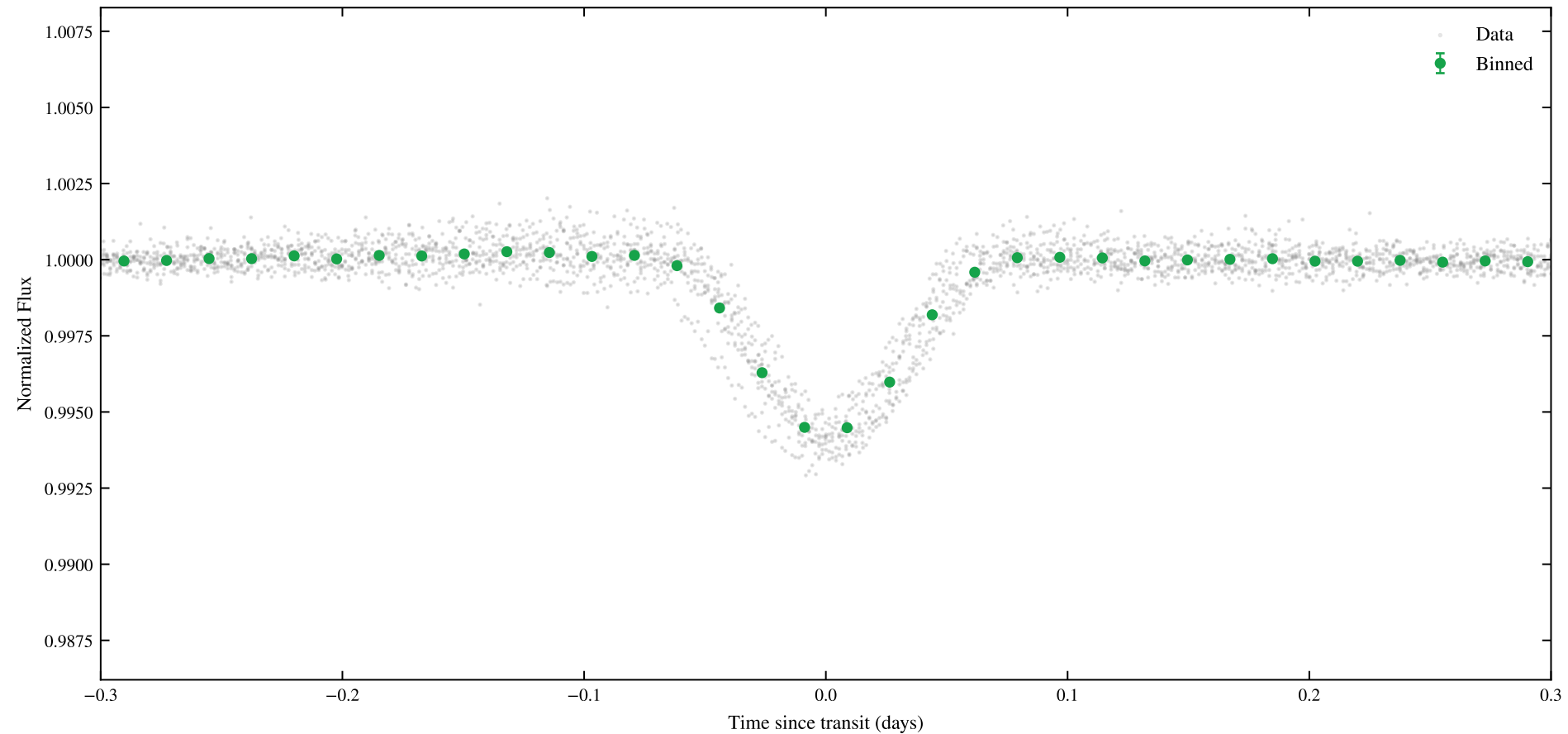
TIC 128790976 | Sectors: 13 | Phase-Folded Transit (P = 3.51948 d)
