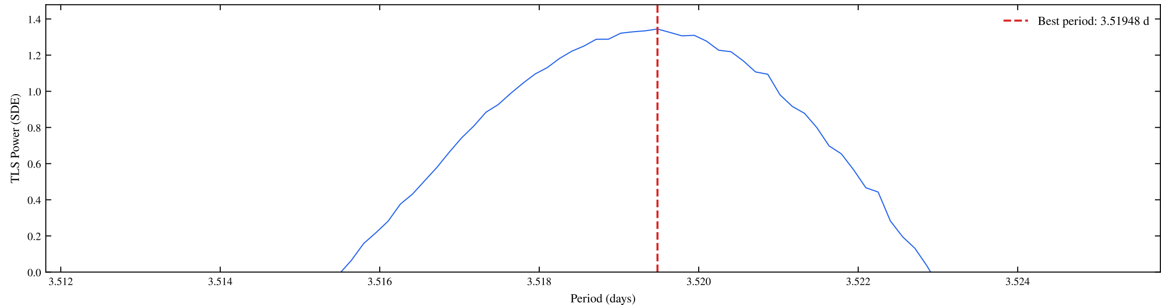
TIC 128790976 | Sectors: 13 | TLS Coarse Periodogram (SDE = 1.34)
